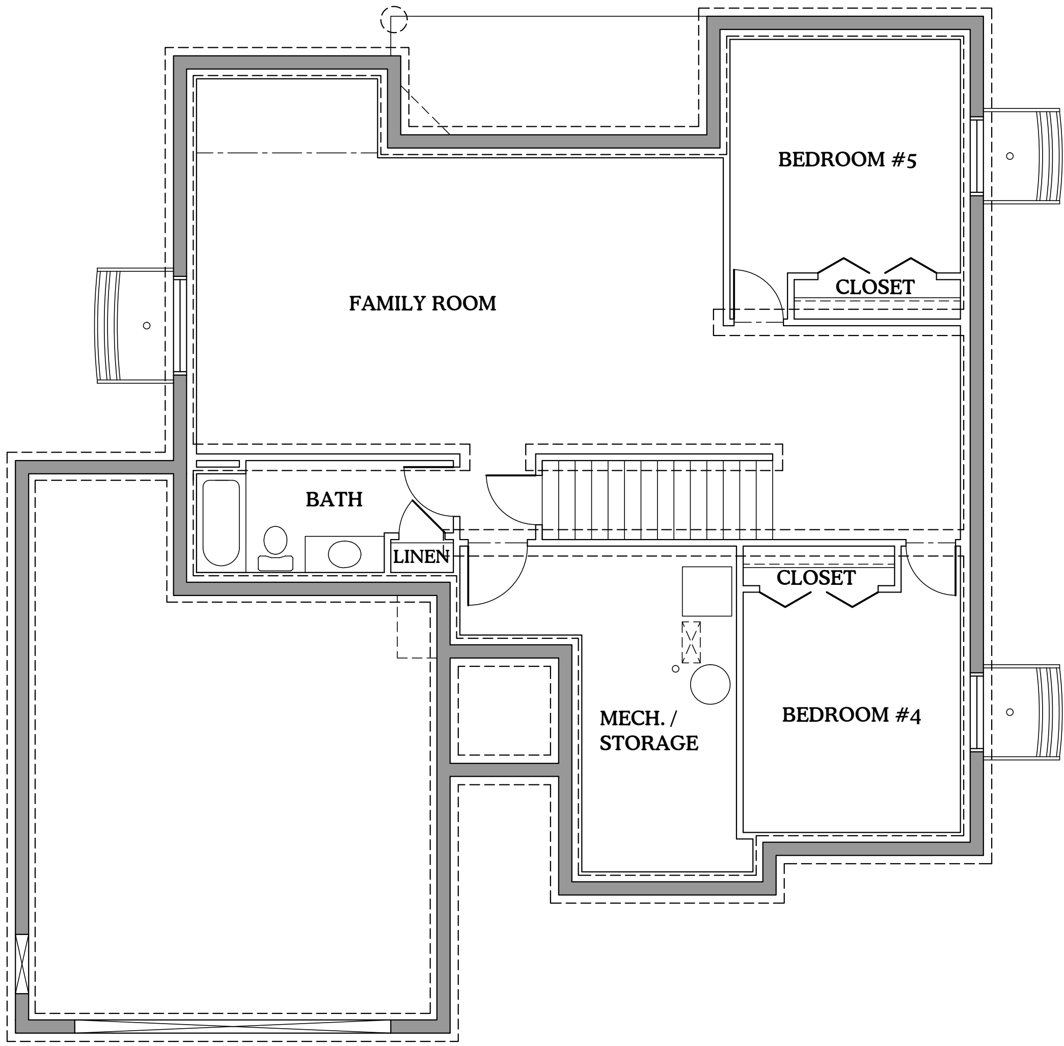
BASEMENT PLAN
